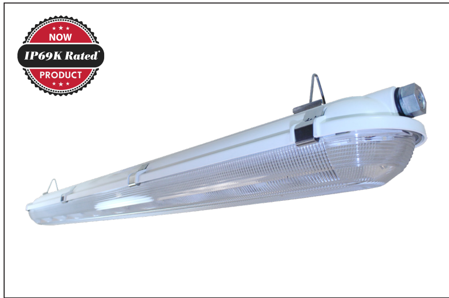
4SNGPG50 parking garage lens, DC-2S die cast end plug and LSS-5 stainless steel latches shown.
