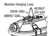
Modular Hanging Loop
