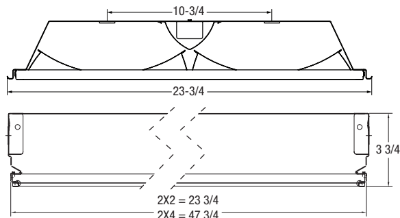
ELC Cross Section
