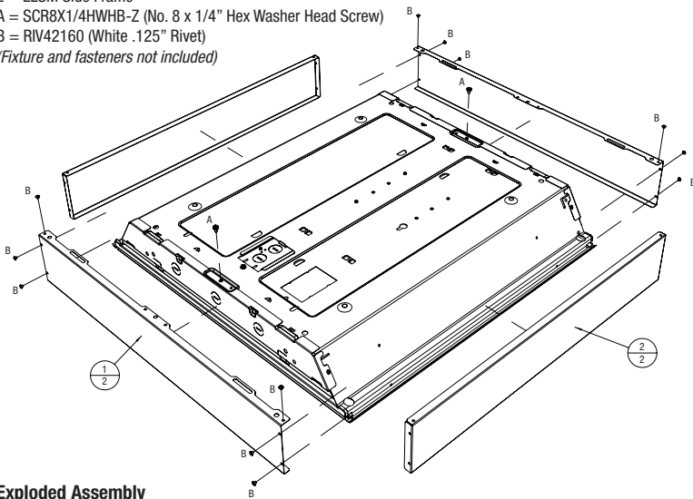
Exploded Assembly
