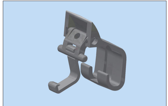
Figure 2. Assembled latch
