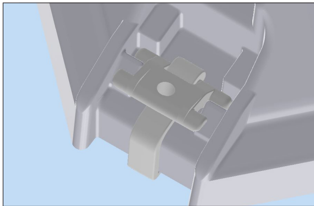
Figure 3. Minor hook and hook connector placement
