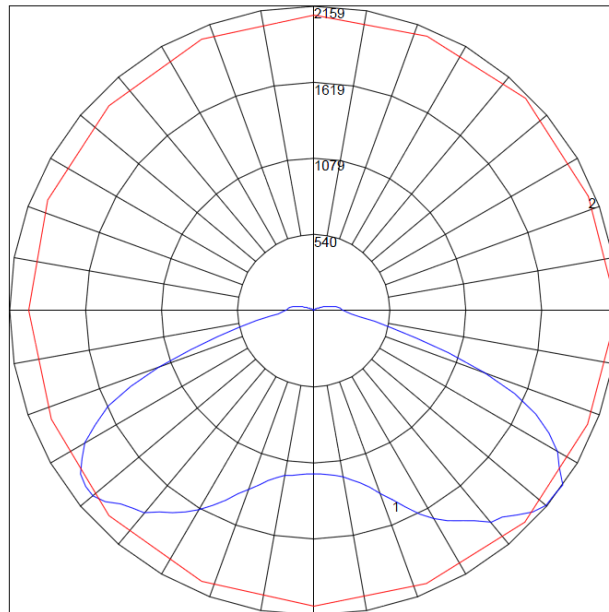
Maximum Candela = 2158.8 Located At Horizontal Angle = 0, Vertical Angle = 55 # 1 - Vertical Plane Through Horizontal Angles (0 - 180) (Through Max. Cd.) # 2 - Horizontal Cone Through Vertical Angle (55) (Through Max. Cd.)
